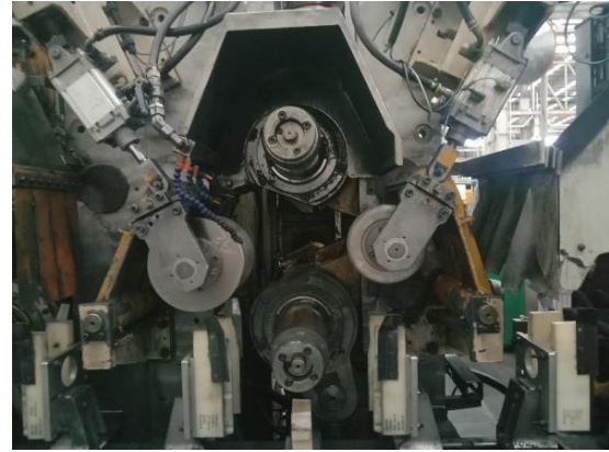
Gambar 4 Roll former dan side guide
