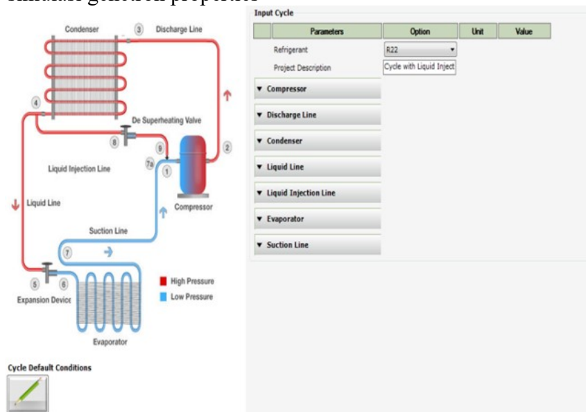
Gambar 3.3 Simulasi software genetron properties
