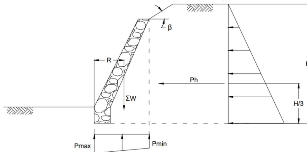
Gambar 6. Desain Dinding Penahan Tipe 2
